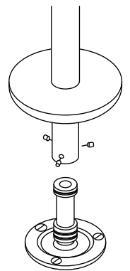
Base for floor mounting.
